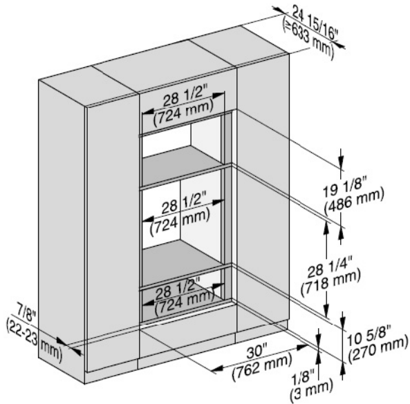
Isometric View
