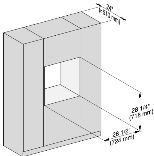
Isometric View
