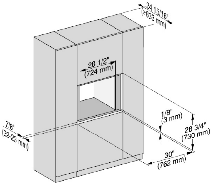
Isometric View
