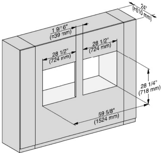
Isometric View
